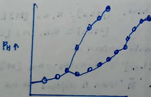
Potentiometric titration of s -sulphosalicylic acid ( \text{H}_2\text{S} ) in the presence of \text{CuSO}_4
